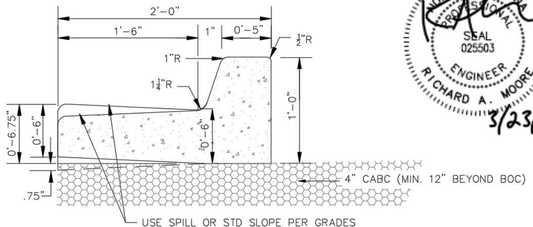
STANDARD 24" CURB SECTION
