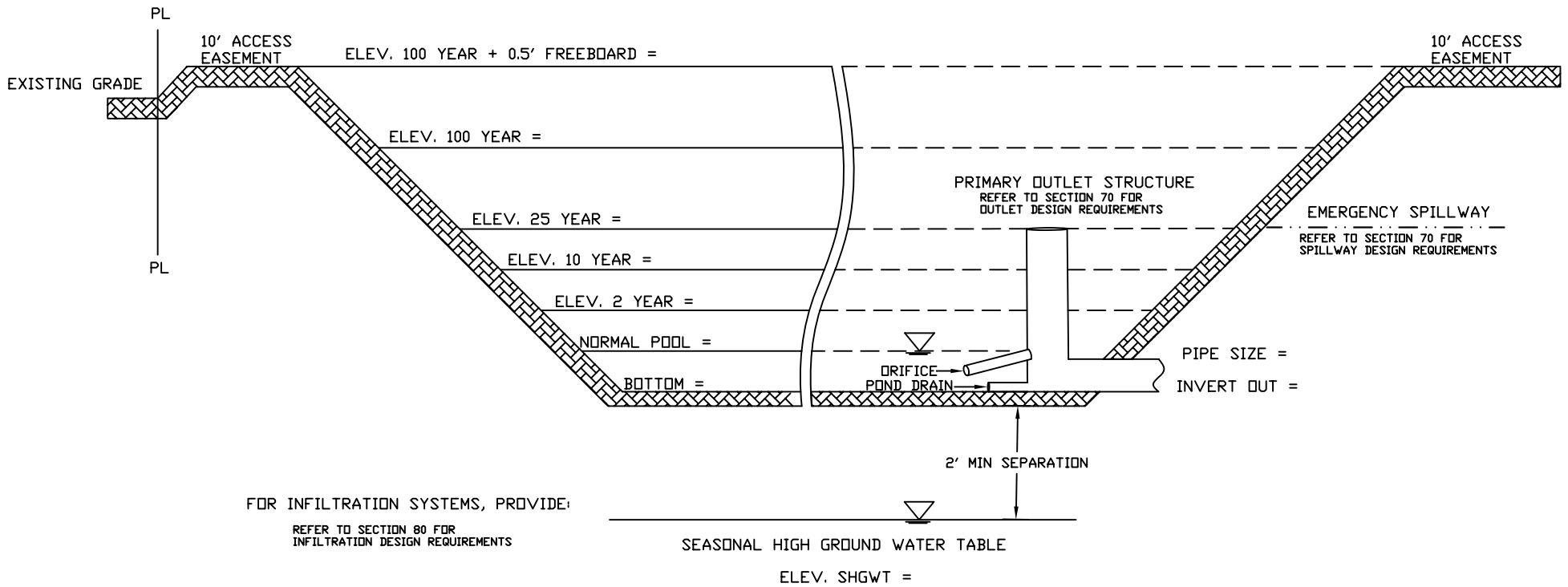
FIGURE 70-1 NHC POND DETAIL
